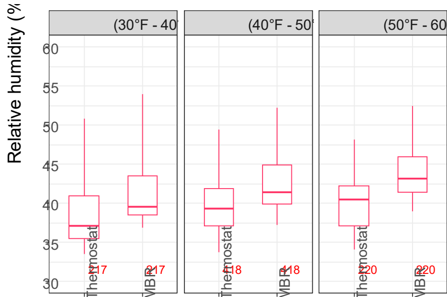
Figure 39. Variation in relative humidity at different measurement locations and different hourly average outdoor temperature bins – during heating
