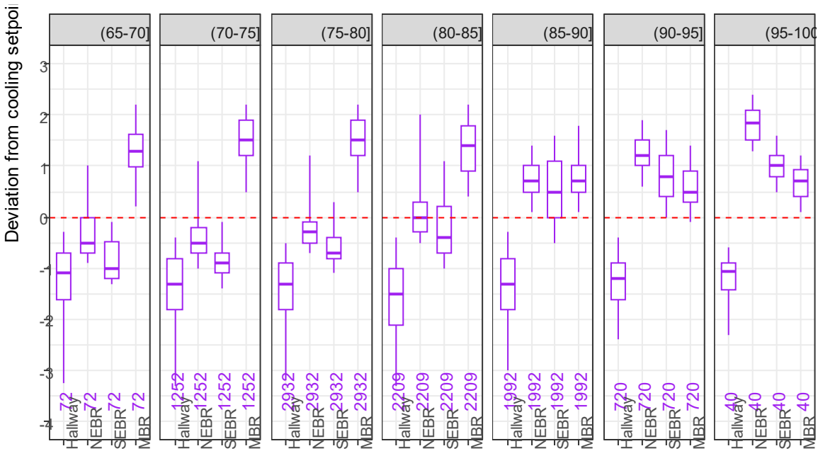
Figure 46. Room temperature deviation from cooling setpoint temperature in different hourly average outdoor temperature bins – heat pump cooling period with floor duct setup
