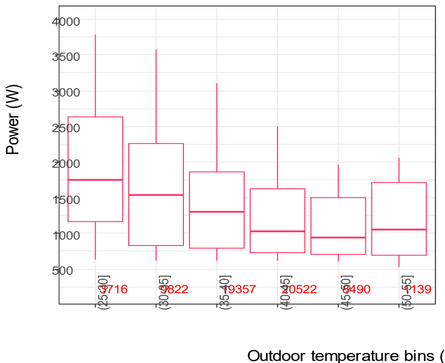
Figure 12. Hourly average heat pump (heating mode) power grouped in 5°F hourly average outdoor-temperature bins. Groups of fewer than 100 points are excluded.
