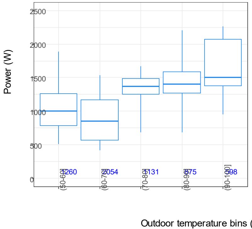
Figure 13. Heat pump (cooling mode) power in 10°F hourly average outdoor-temperature ranges (using one-minute data)
