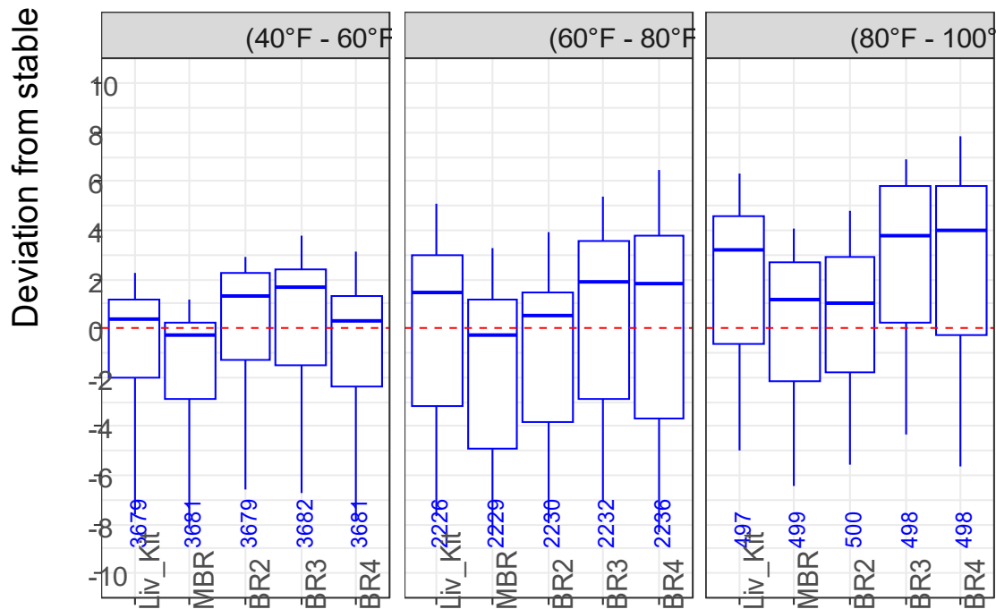
Figure 24. Hourly average room-wise temperature deviation from stable cooling setpoint temperature in hourly average outdoor temperature bins—heat pump cooling period. Includes data for days with the thermostat set in cooling mode.
