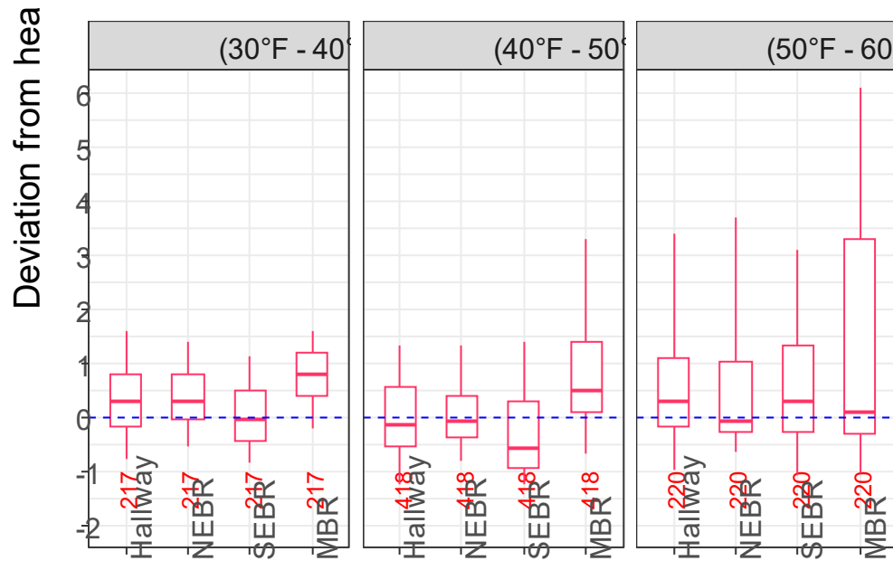
Figure 37. Room-wise temperature deviation from heating setpoint temperature in different hourly average outdoor temperature bins – heat pump heating period
