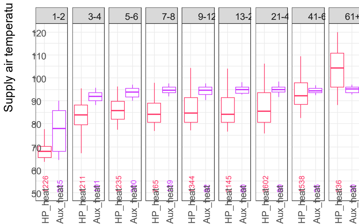
Figure 26. Supply air temperature variations during various time steps (in minutes) of the heat pump heating cycle
