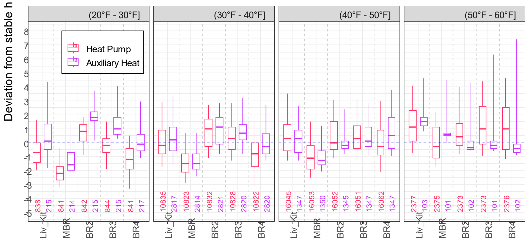
Figure 23. Hourly average room-wise temperature deviation from stable heating setpoint temperature in outdoor temperature bins – heat pump and auxiliary heat. Includes data for days with the thermostat set to heating control mode.
