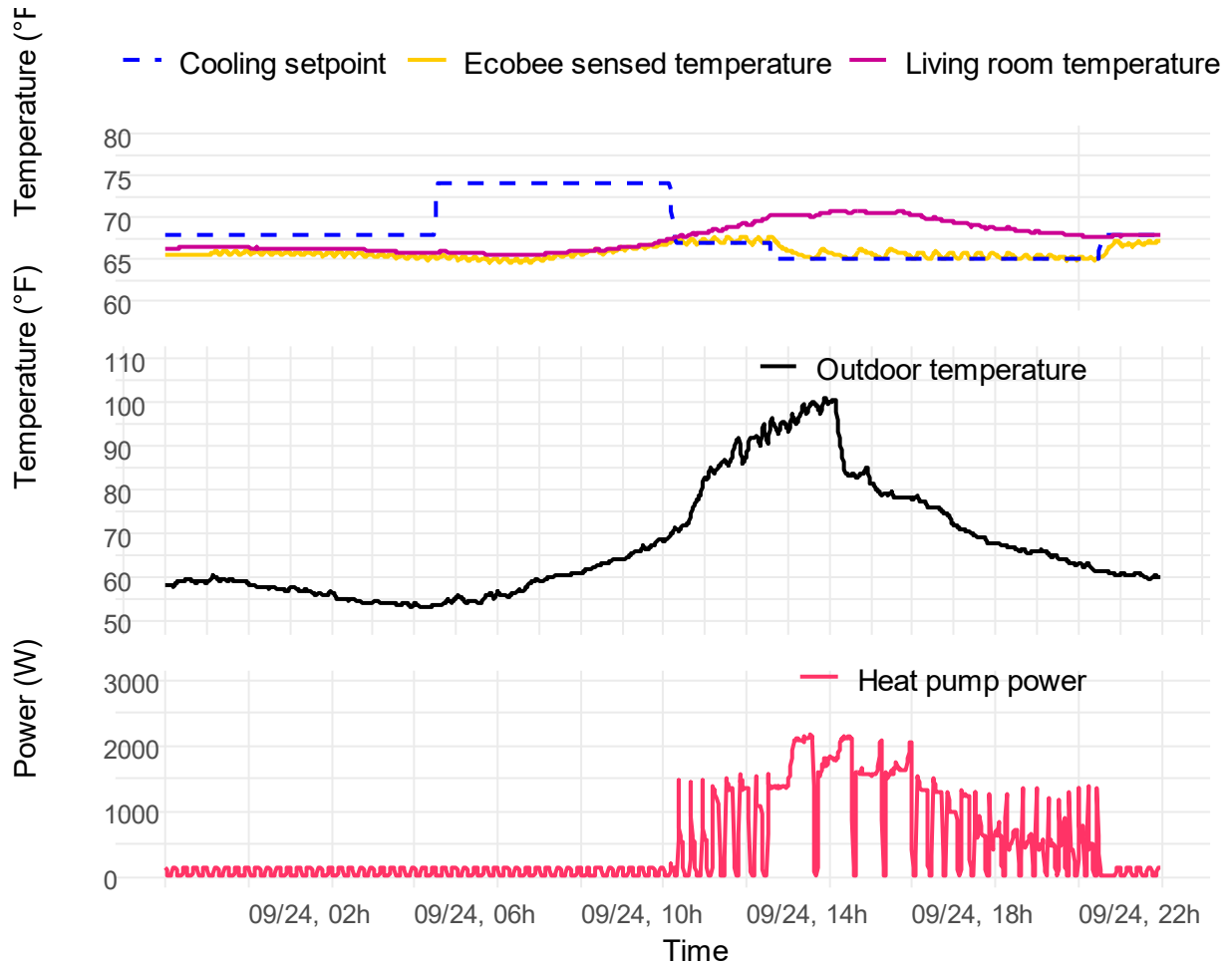
Figure 8. Example of heat pump operation in cooling mode
