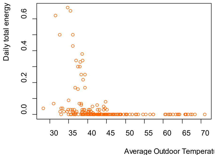
Figure 19. Daily total energy consumption (kWh) during crankcase heat operation vs average outdoor temperature
