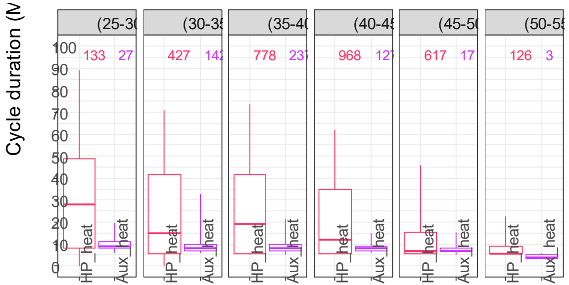
Figure 14. Heat pump heating and auxiliary heat cycle duration 5°F hourly average outdoor-temperature ranges (using one-minute data). The numerical values within each box represent the number of heating cycles
