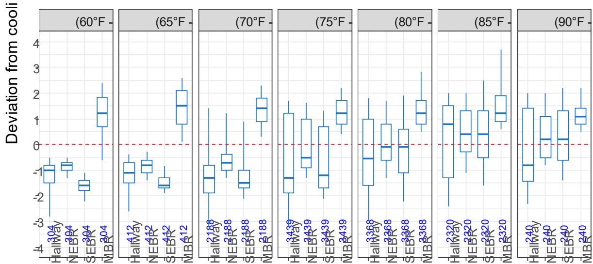
Figure 36. Room-wise temperature deviation from cooling setpoint temperature in different hourly average outdoor temperature bins – heat pump cooling period
